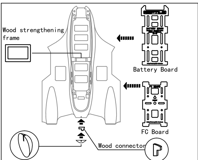
Installation mode of engine room equipment board.
