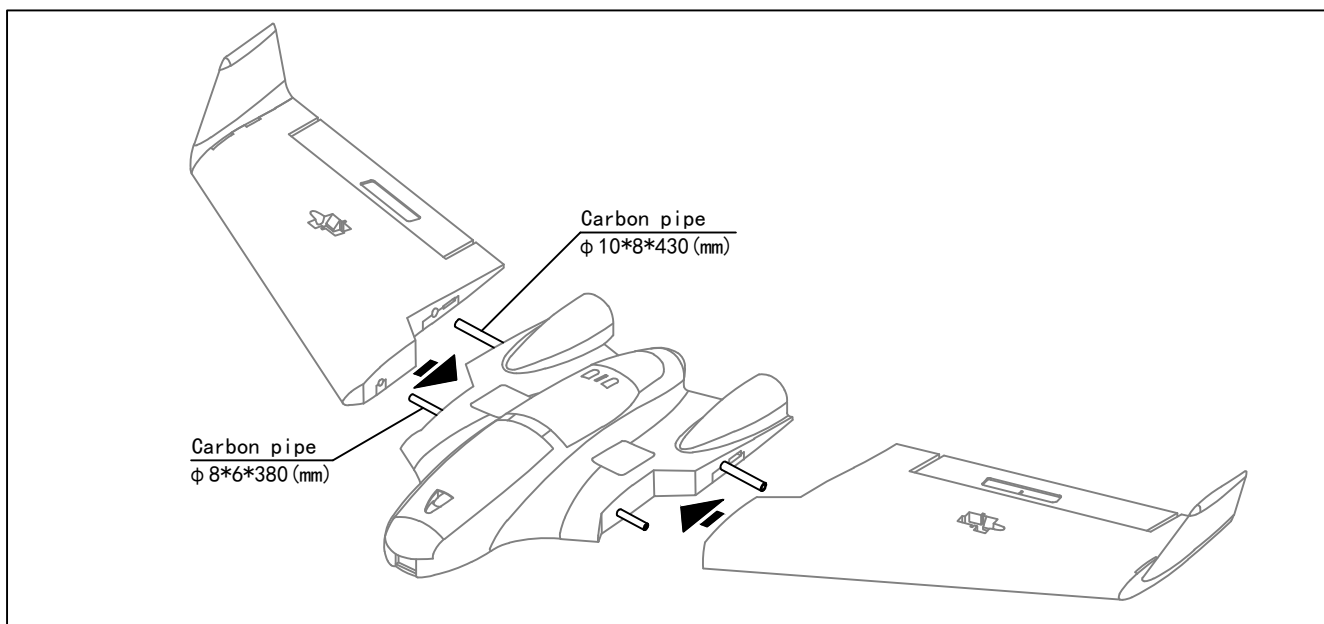
Carbon tube links for airframe and wing. The airframe and the wing are locked by the plastic pipe clamp.
