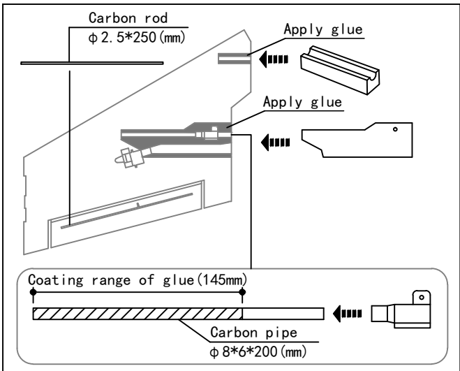
Installation mode of carbon tube for wing.
