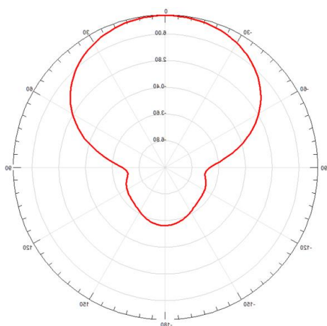
Surface radiation pattern
