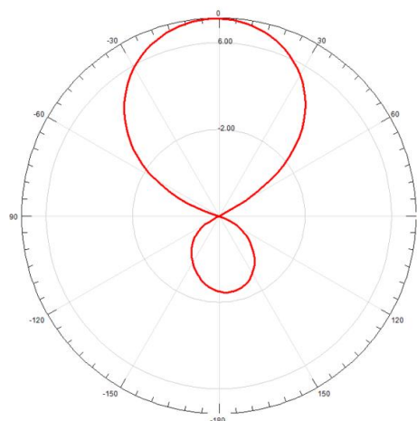
Vertical plane radiation pattern
