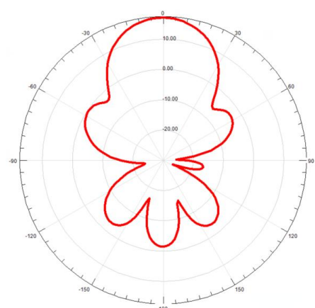
Vertical plane radiation pattern
