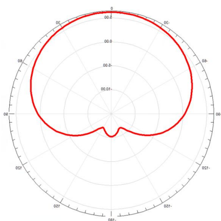
Surface radiation pattern
