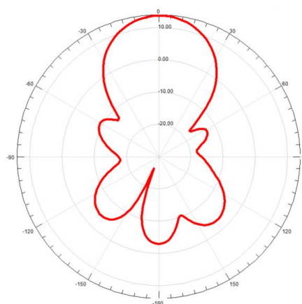
Vertical plane radiation pattern
